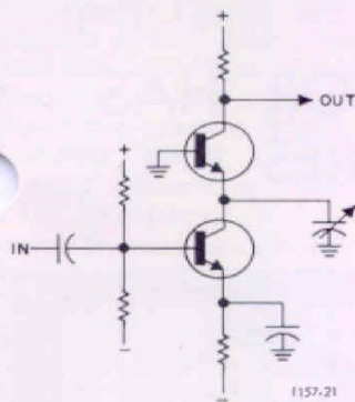
Figure 5. Simplified schematic diagram of the emitter-peaked cascode amplifier.
