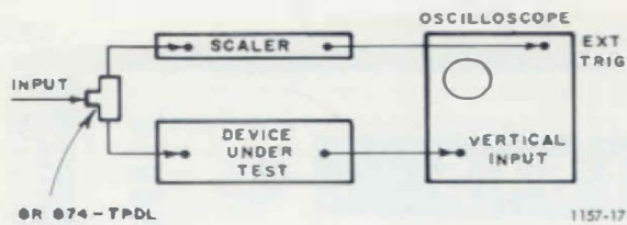
Figure 2. Use of the 1157 Scaler to trigger an Oscilloscope.
