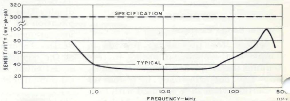
Figure 3. Typical and specified peak-to-peak sine-wave input voltage required to drive the 1157 Scaler.
