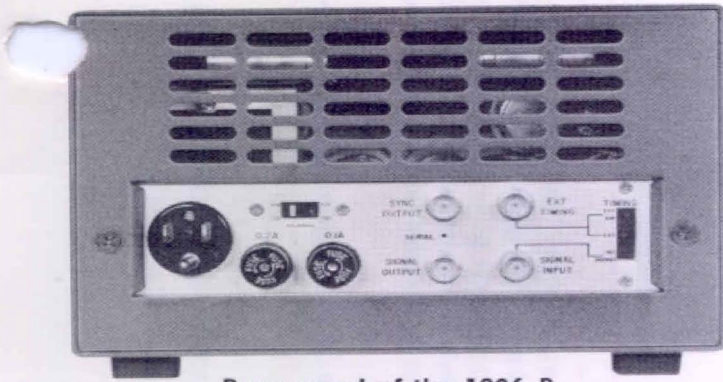
Rear panel of the 1396-B.
