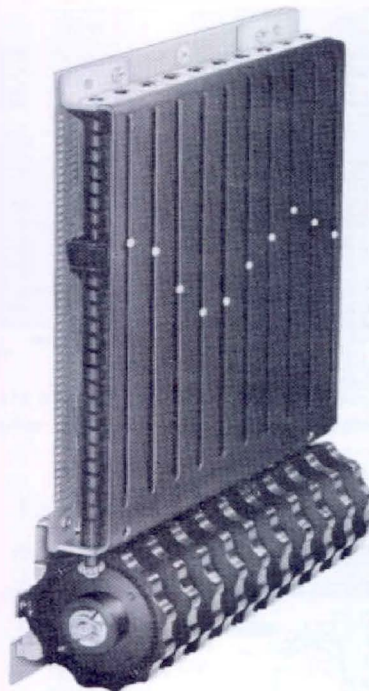
Figure 3. An assembly of ten of the adjustable attenuators. The setting of each attenuator is indicated by the vertical position of a dot in the front-panel display.
