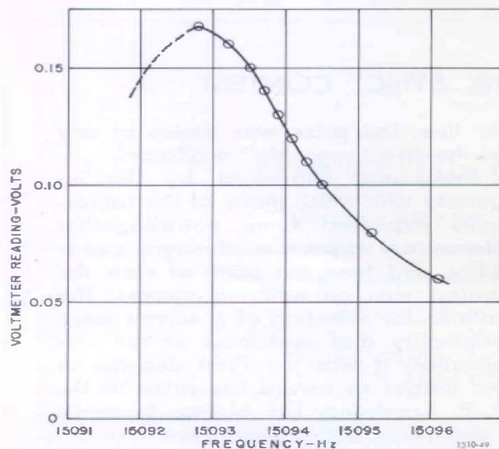
Figure 2. Plot of resonance data for a typical sample. The system turned out to be unstable below resonance, but data for this region could have been obtained, if necessary, by reversing connections somewhere in the loop.
