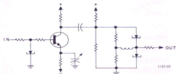
Figure 6. High-speed flip-flop — simplified schematic diagram.
