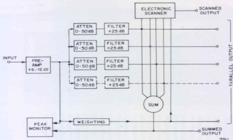
Figure 2. Block diagram of the multi-filter.
