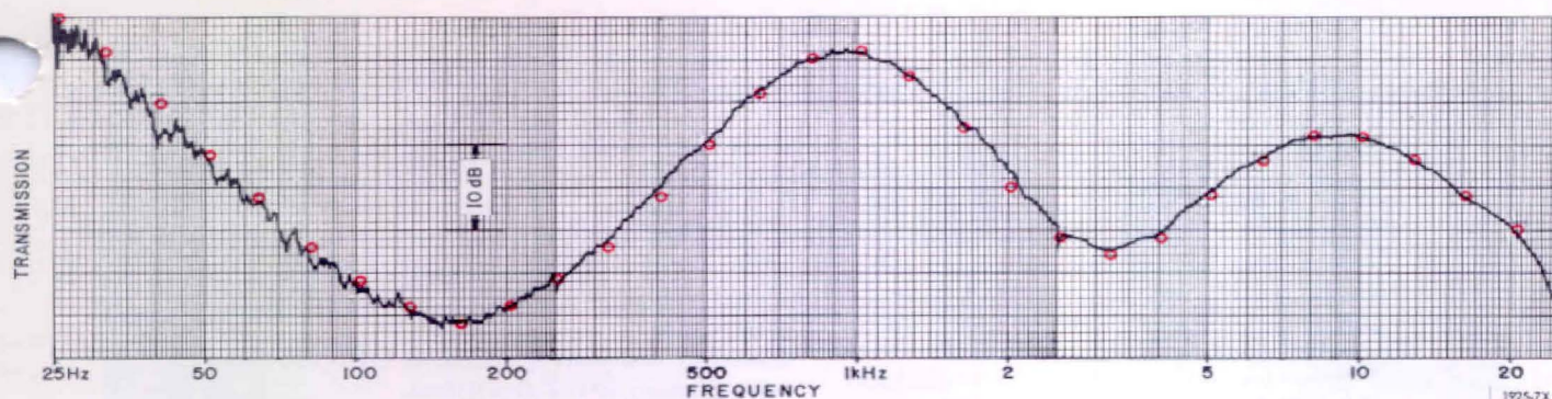
Figure 5. A more likely example. When there are no abrupt discontinuities or steep slopes, the \frac{1}{3} -octave analysis (solid black line) departs from the multifilter display by less than the measurement error.
