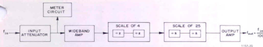
Figure 4. Simplified block diagram of the 1157 Scaler.
