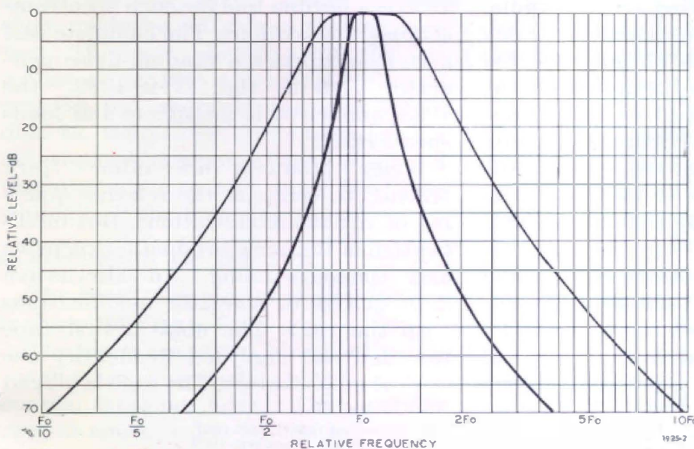
Figure 1. Octave and 1/3-octave filter characteristics.
